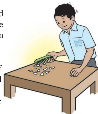
10.9 : Electrostatic force
