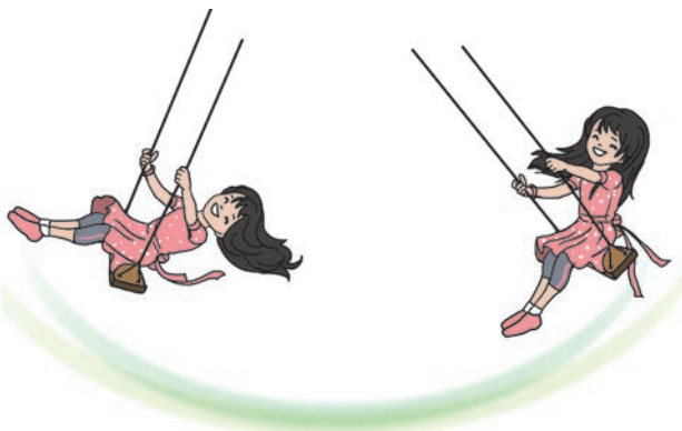
9.5 : Oscillatory motion
