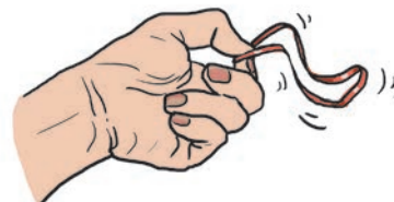
5.10 : Elasticity
