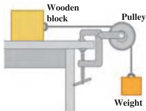
7.4 Work
