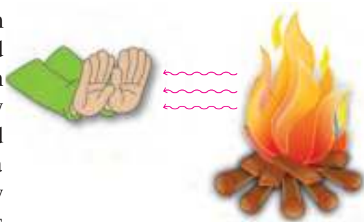
9.5 Radiation
