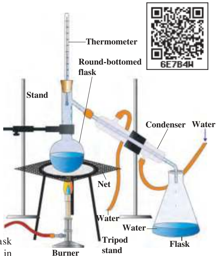
14.4 Distillation method
